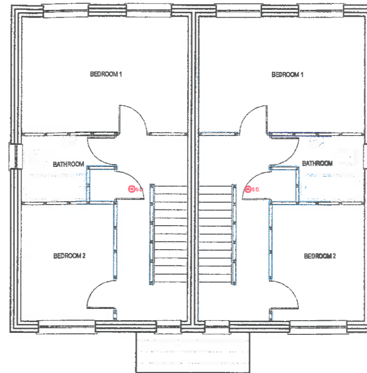
PROPOSED FIRST FLOOR PLANS
