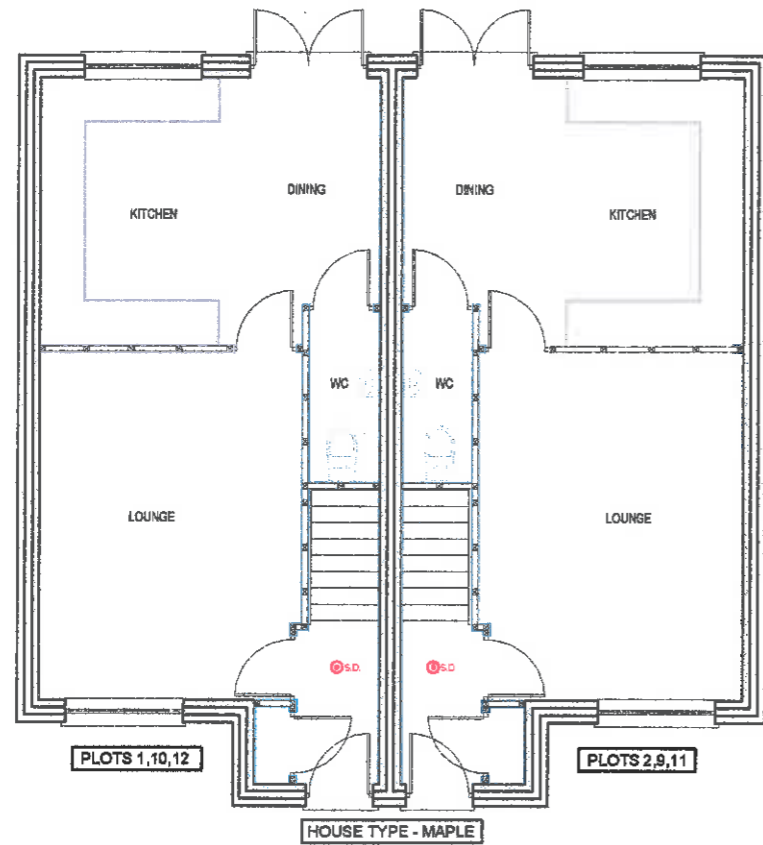
PROPOSED GROUND FLOOR PLANS
