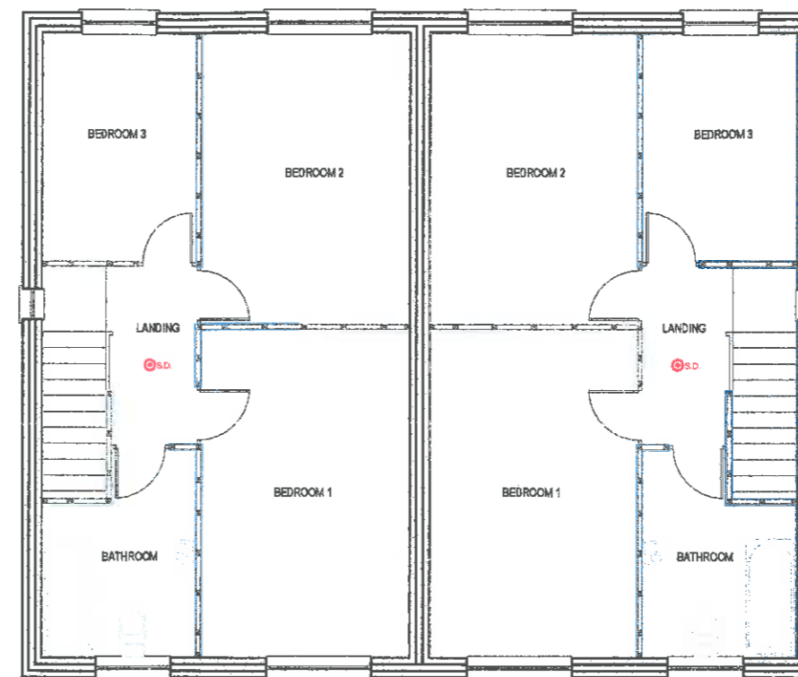
PROPOSED FIRST FLOOR PLANS
