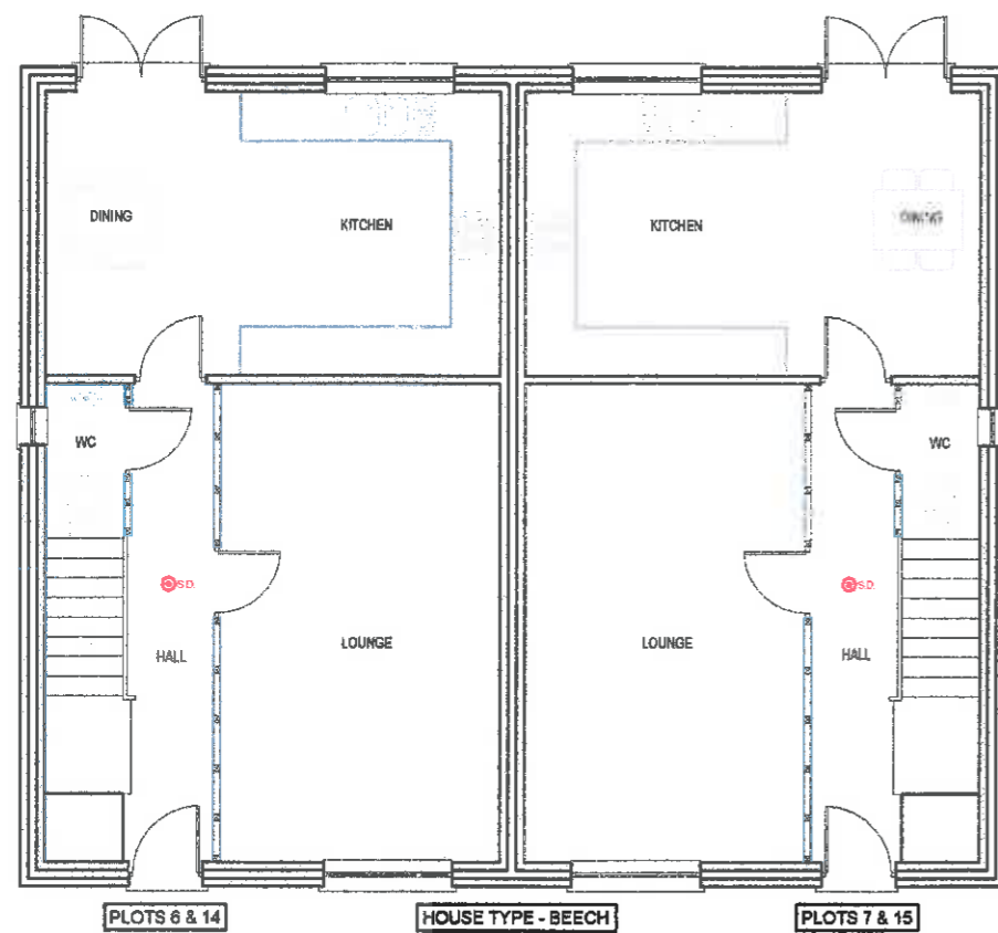
PROPOSED GROUND FLOOR PLANS
